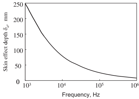
Figure 5. Skin effect depth in the fiber direction of a widely used CFRP.
