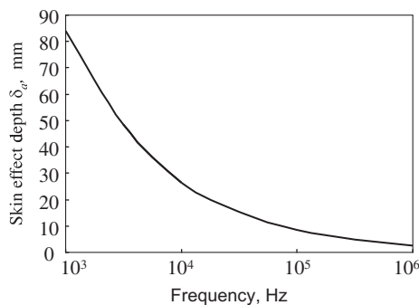
Figure 4. Skin-effect depth of IM600/133 in the fiber direction.
