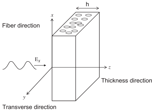
Figure 1. Simple model of uniform electric current in a conductive slab.
